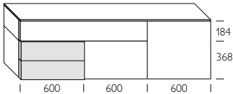
Open configuration
