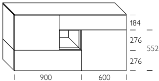
Open configuration
